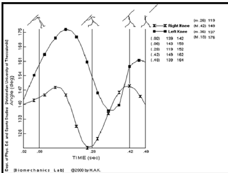
Figure 4. Javelin throwing pattern with a stretch-shortening function of the knee extensor muscles of both legs during the double support of the delivery phase (m: minimum value; M: maximum value). From left to right, the three vertical axis represent the instances of last right foot touchdown, the last left foot touchdown and the release of the javelin, as indicated by the respective stick figure at the top of the plot.
